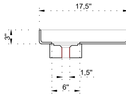
Sink Section
