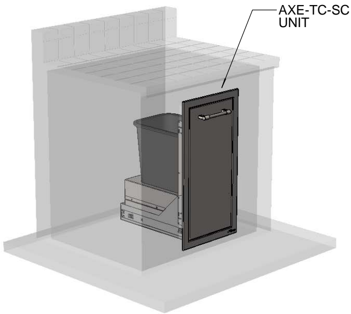
TYPICAL AXE-TC-SC INSTALLATION
