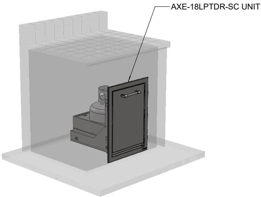
TYPICAL AXE-18LPTDR-SC TANK DRAWER INSTALLATION
