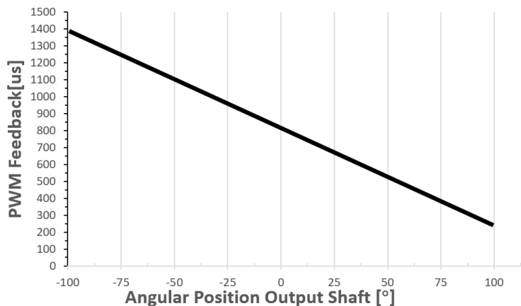
Position Feedback
