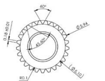
6mm25T Output Shaft Spline
