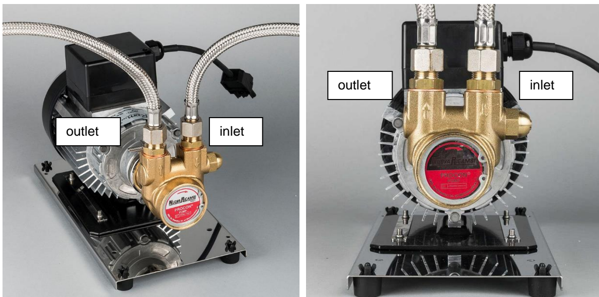
Figure I 2. Pump with inlet and outlet shown.
