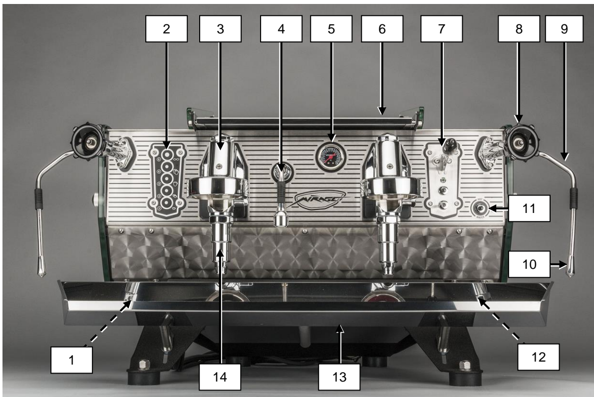
Figure W 1. Showing main operational parts of the Mirage Duetto equipped with optional pre-infusion cylinders. Special show model with touchpad operation for the left group and bastone operation for the right group. The Mirage Triplette is wider since it has an extra group in between the two groups shown here but its function is identical to a Duetto.
