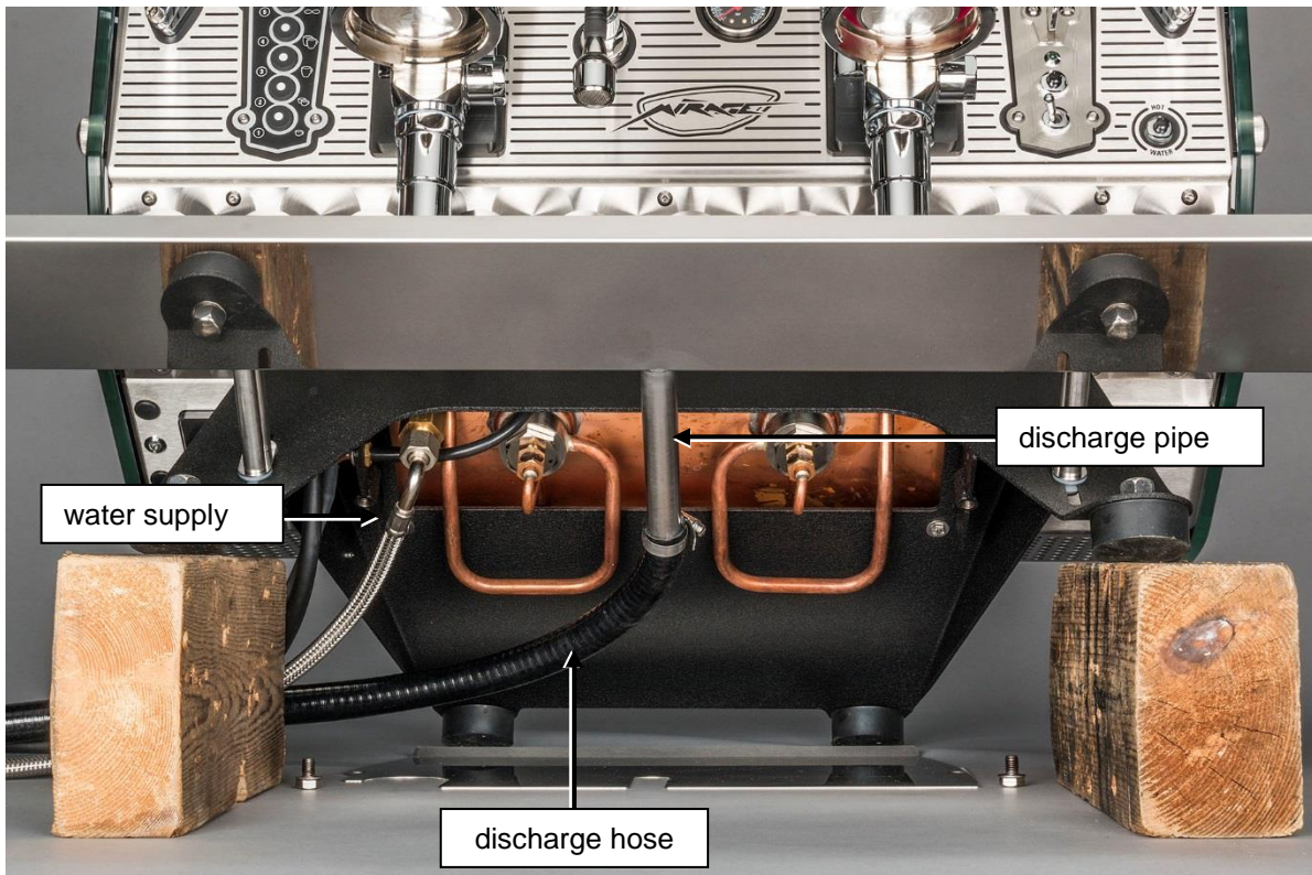
Figure I 3. Mirage Duetto tilted backwards by use of 2 wooden blocks and bottom panel removed to show high pressure water supply and discharge hose pushed on discharge pipe. Blocks have dimensions HxWxD = 15x5x20 cm; 6x2x8 inch.
