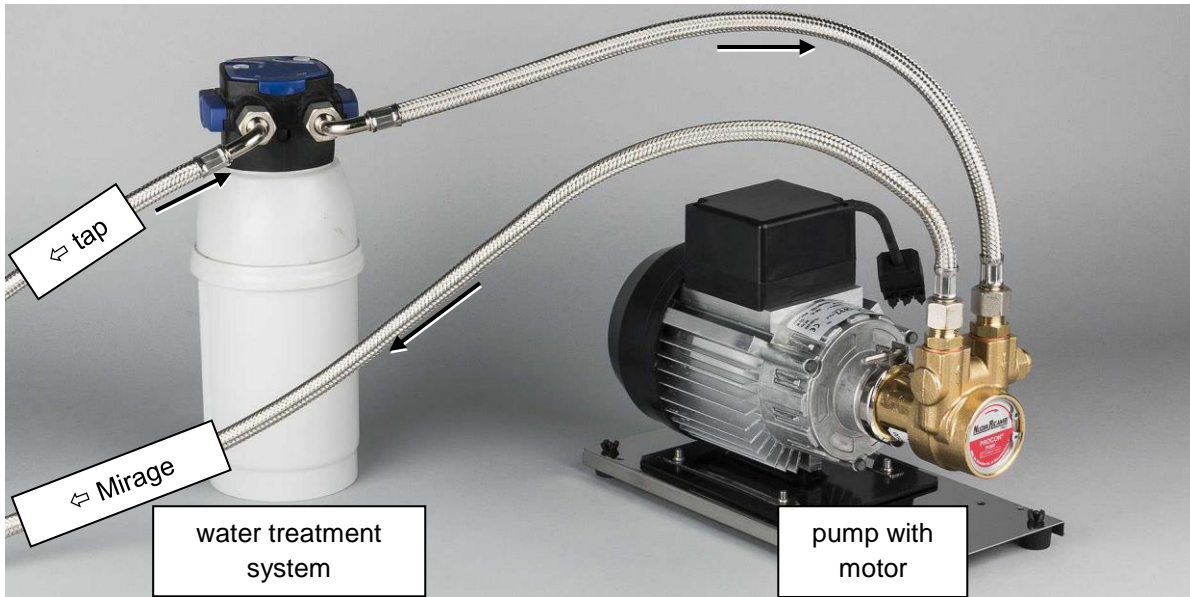
Figure I 1. Water treatment system (not included) on left is connected to the pump on the right. Water flow is according to arrows. Tap and Mirage will be to left of figure.
