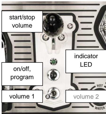
Figure U 3. Functions of a bastone unit of a Mirage. The toggle switch is in the left position, when the bastone is pressed shortly, the brew will automatically stop after pre-set volume 1 has passed the flow meter.
