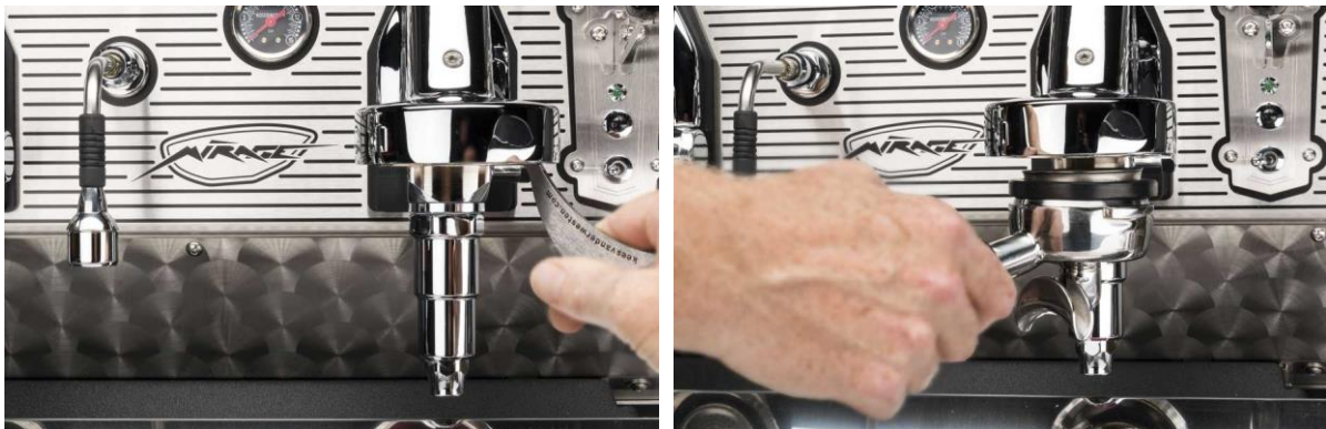
Figure U 6 (left). Pry left and right with group screen extractor to remove group screen and ring.
