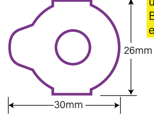
Shape 32 same shape as 3M 1692 used on Mr. Blue/Orange edgers
