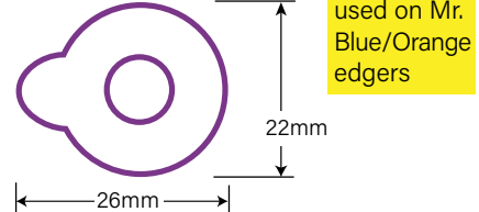
Shape 36 same shape as Gam 403 used on Mr. Blue/Orange edgers
