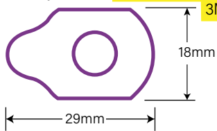
Shape 31 (same shape as 3M 1712N & 3M 1712NR)
