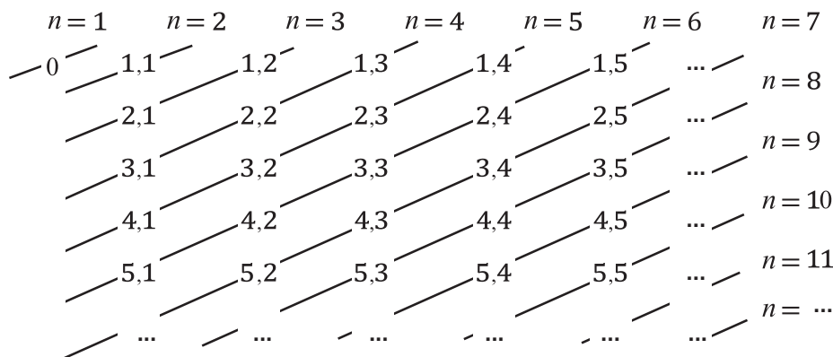
Figure 19. The integers and rational numbers are countable. ■
