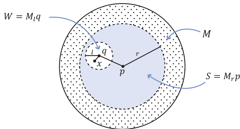
Figure 13. The r -neighborhood of p is an open set, because q is within r . Hence, S is open.
