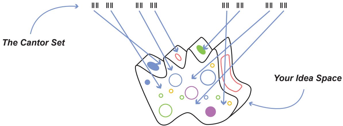
Figure 23. Your idea space is uncountable and has zero measure, like The Cantor Set.
