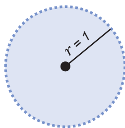
(a) Open Disc.
