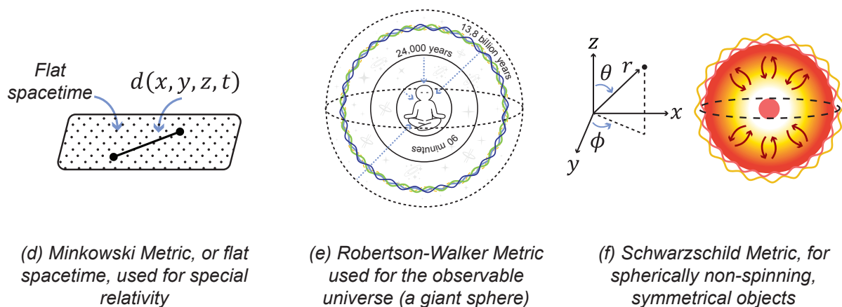
Figure 7. Examples of metric spaces in physics.
