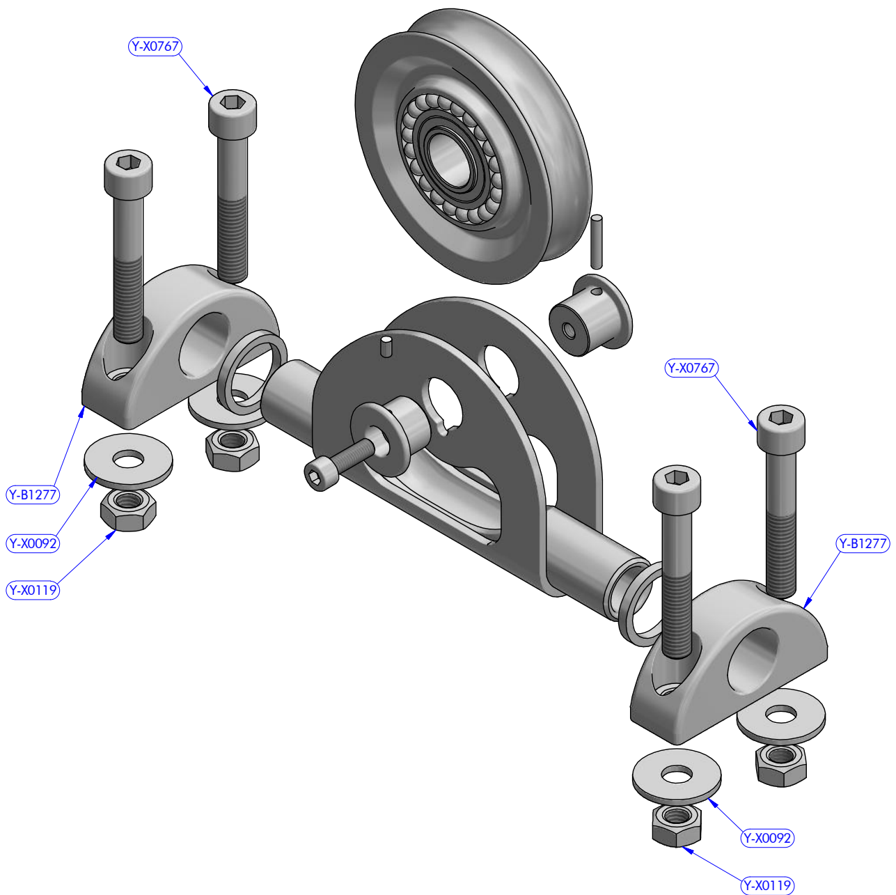
PART LIST 816.075
