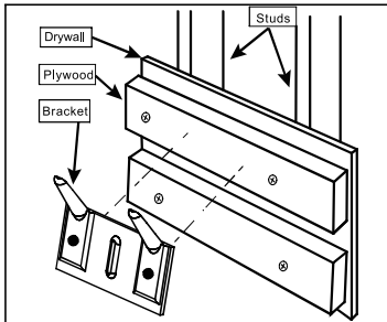
Figure - Mounting for Drywall
