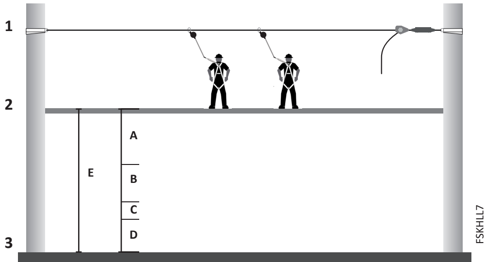
Figure 7: Kernmantle HLL with SRD Minimum Required Fall Clearance
