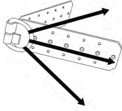
Figure 6: Suitable Load Direction on Roof Anchors
