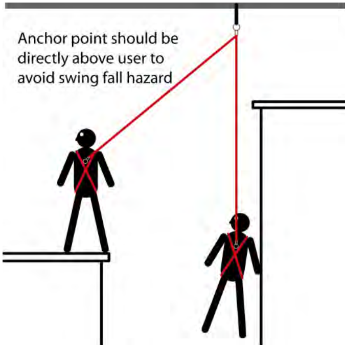
Figure 2.2: Swing-Fall Diagram
