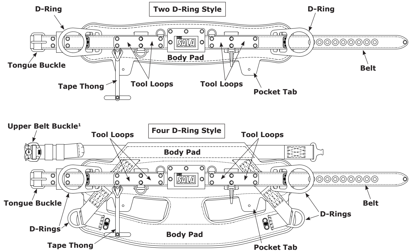
Figure 1 - DBI-SALA Lineman's Belts
