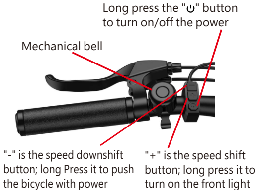
Figure 4 (Left Handlebar)
