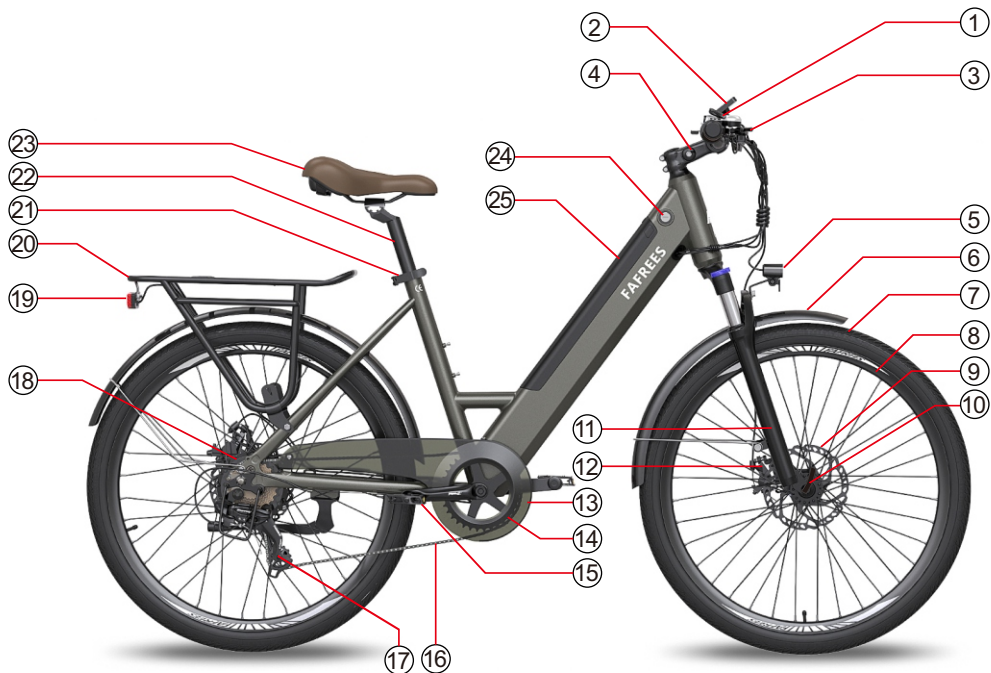
Figure 1 (Bicycle Diagram)
