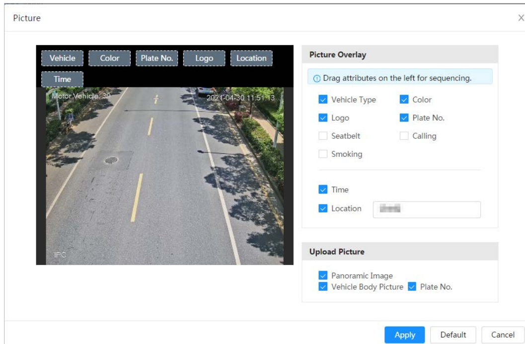
Figure 8-39 Picture
