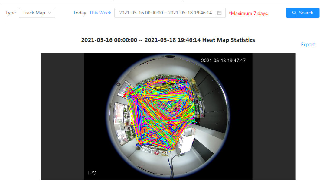
Figure 12-10 Track map
