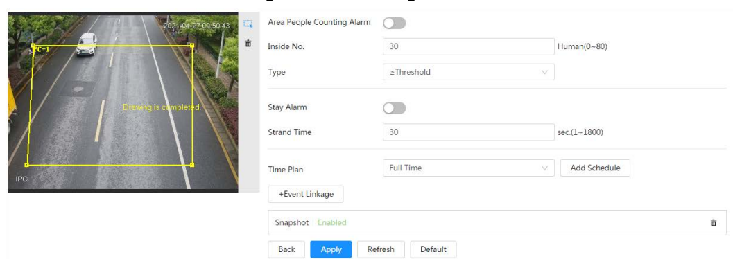
Figure 8-32 Queuing
