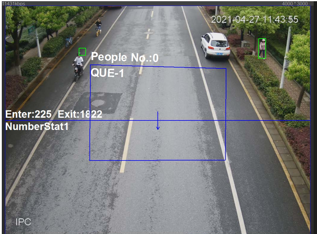
Figure 8-33 Queuing result
