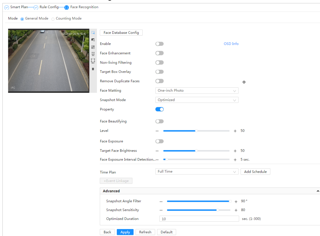
Figure 8-6 Face detection
