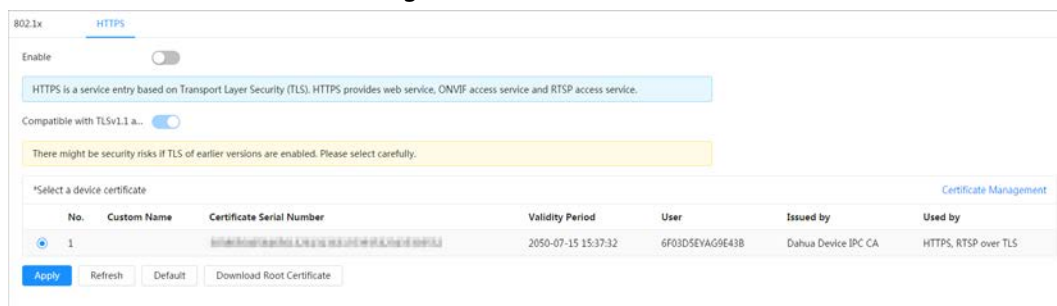
Figure 9-5 HTTPS
