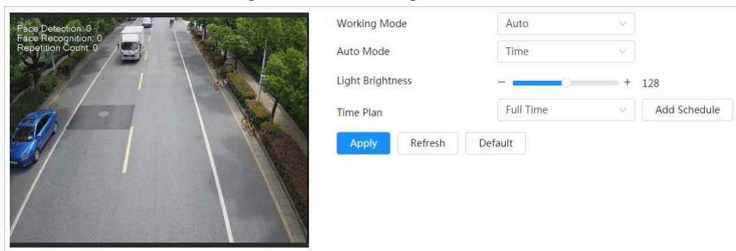
Figure 6-75 External light
