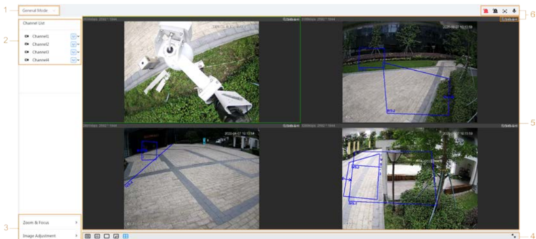
Figure 7-2 Live (multi-channels)
