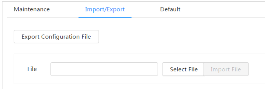
Figure 6-78 Import/Export
