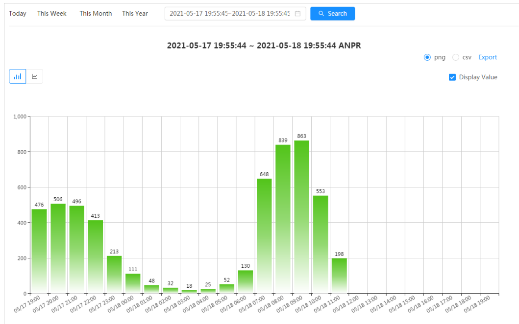
Figure 12-11 ANPR report
