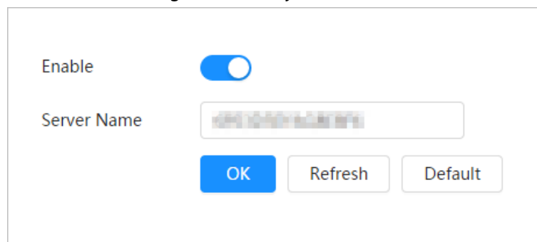
Figure 6-39 Bonjour
