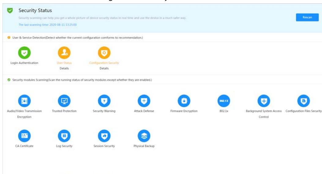
Figure 9-1 Security Status
