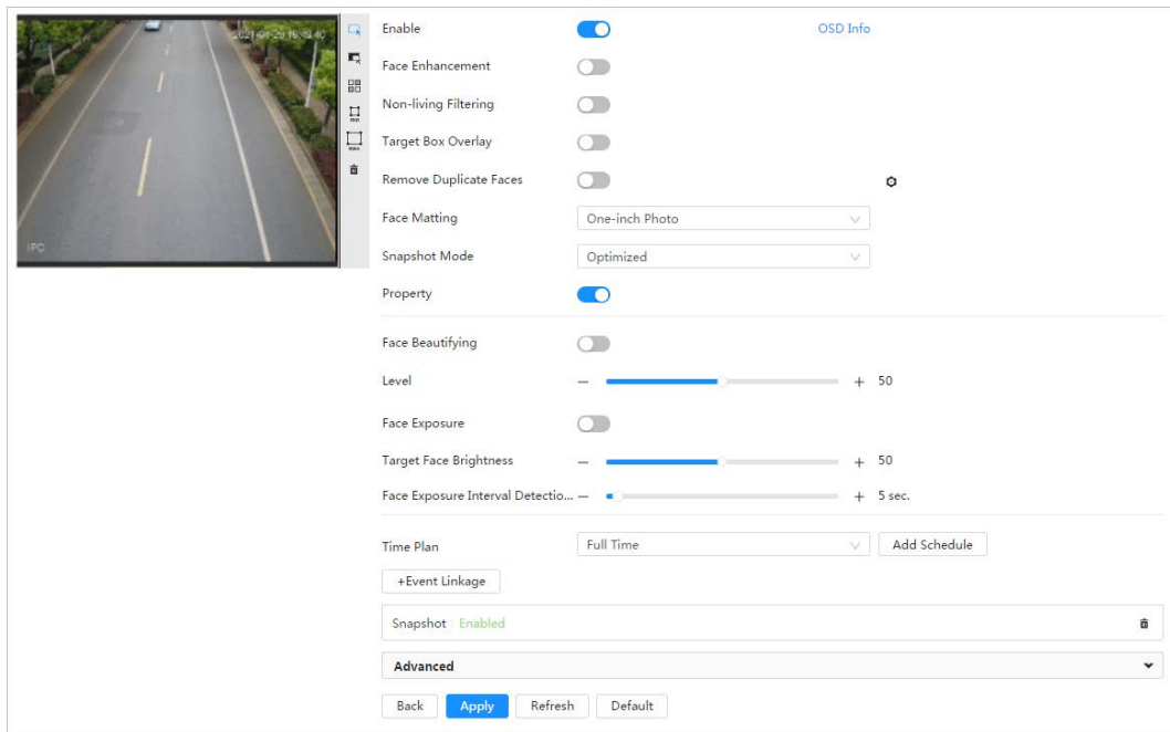
Figure 8-19 Face detection
