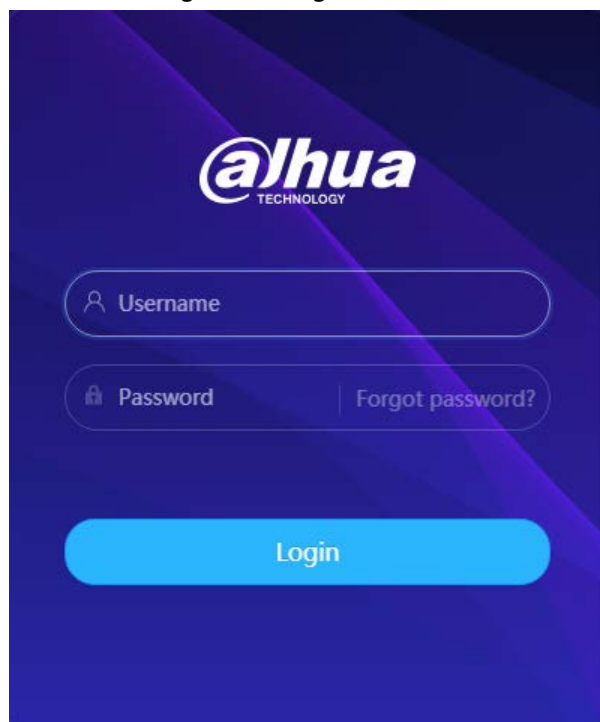
Figure 4-3 Login
