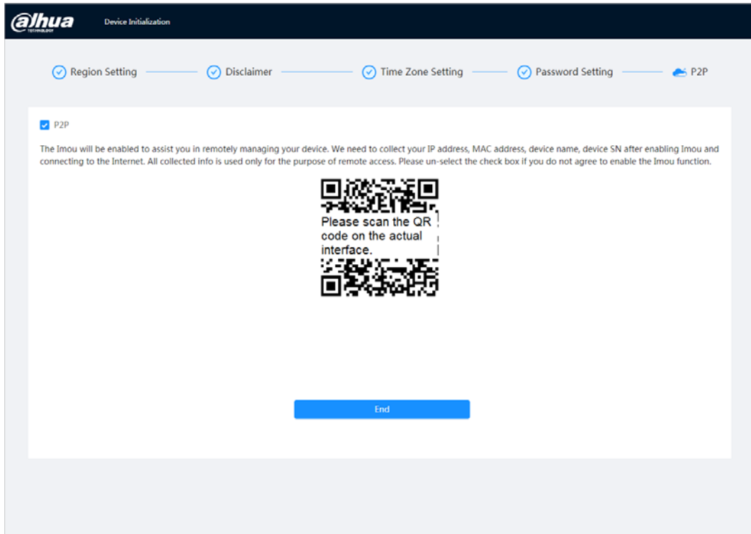
Figure 3-5 P2P
