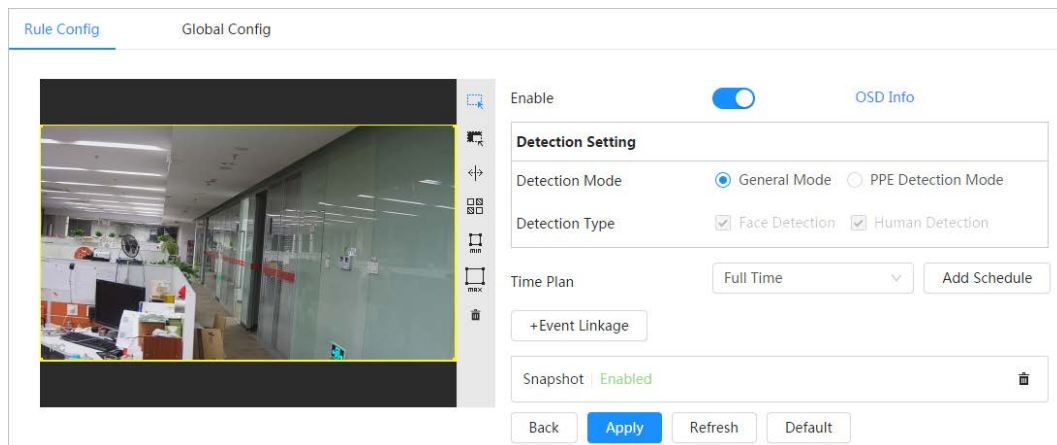
Figure 8-36 Rule configuration
