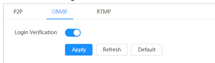
Figure 6-44 ONVIF
