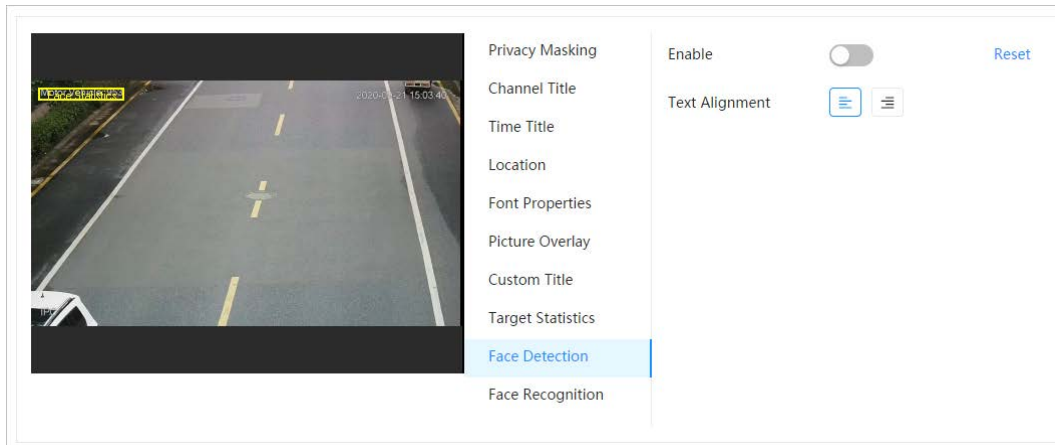
Figure 6-23 Face detection
