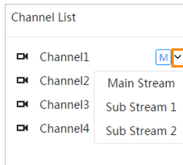
Figure 7-3 Encode bar
