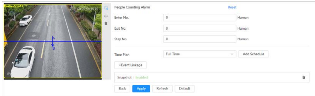
Figure 8-28 People counting
