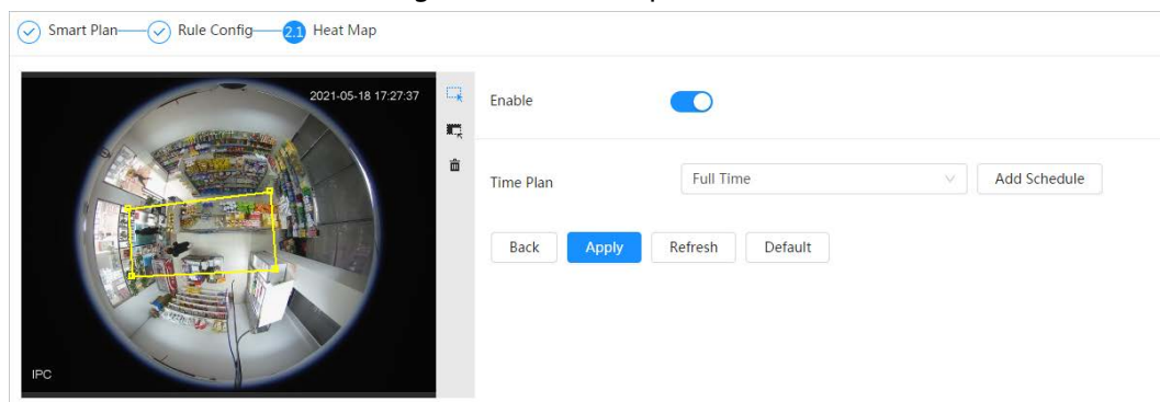
Figure 8-37 Heat Map
