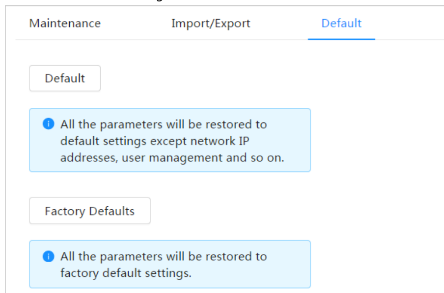
Figure 6-79 Default
