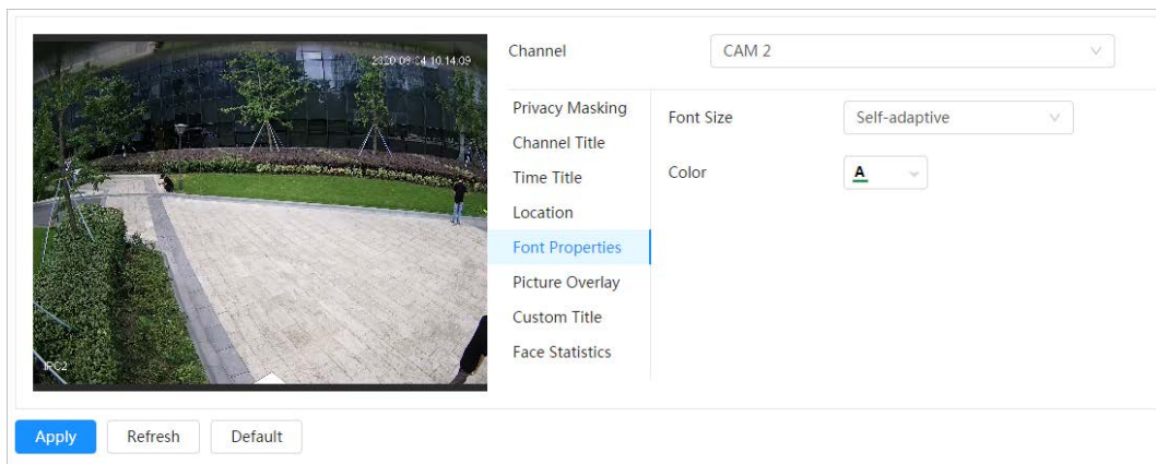
Figure 6-18 Font properties
