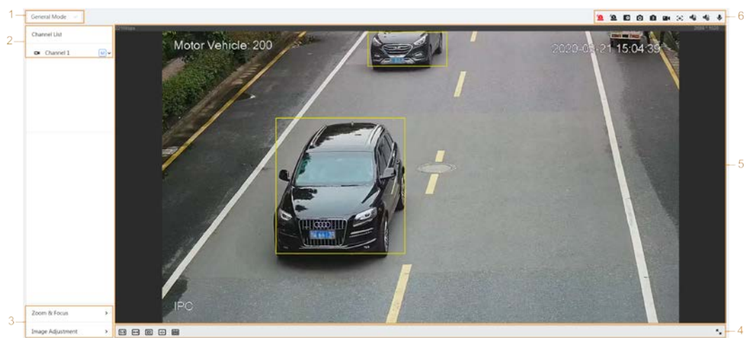
Figure 7-1 Live (single-channel)
