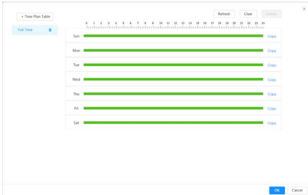
Figure 6-49 Schedule
