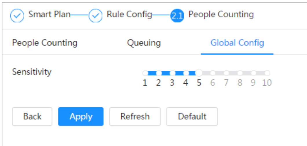
Figure 8-34 Global configuration
