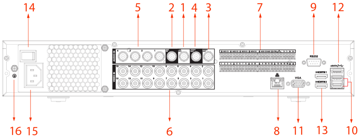
Figure 3-20 Rear panel (3)
