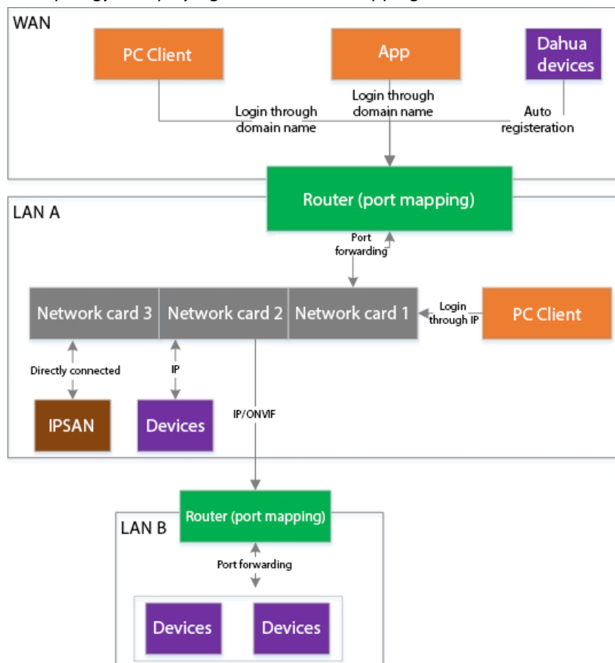
Figure 2-7 Topology of deploying LAN and WAN mapping and dual networks cards
