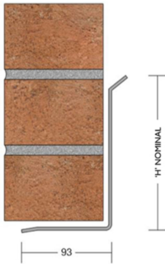
100mm Solid Wall
