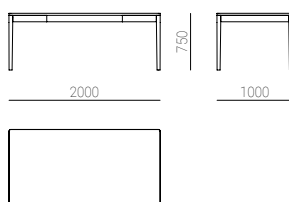
Rectangular 200 x 100
