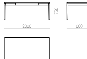
Rectangular 200 x 100
