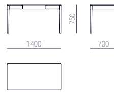
Rectangular 140 x 70
