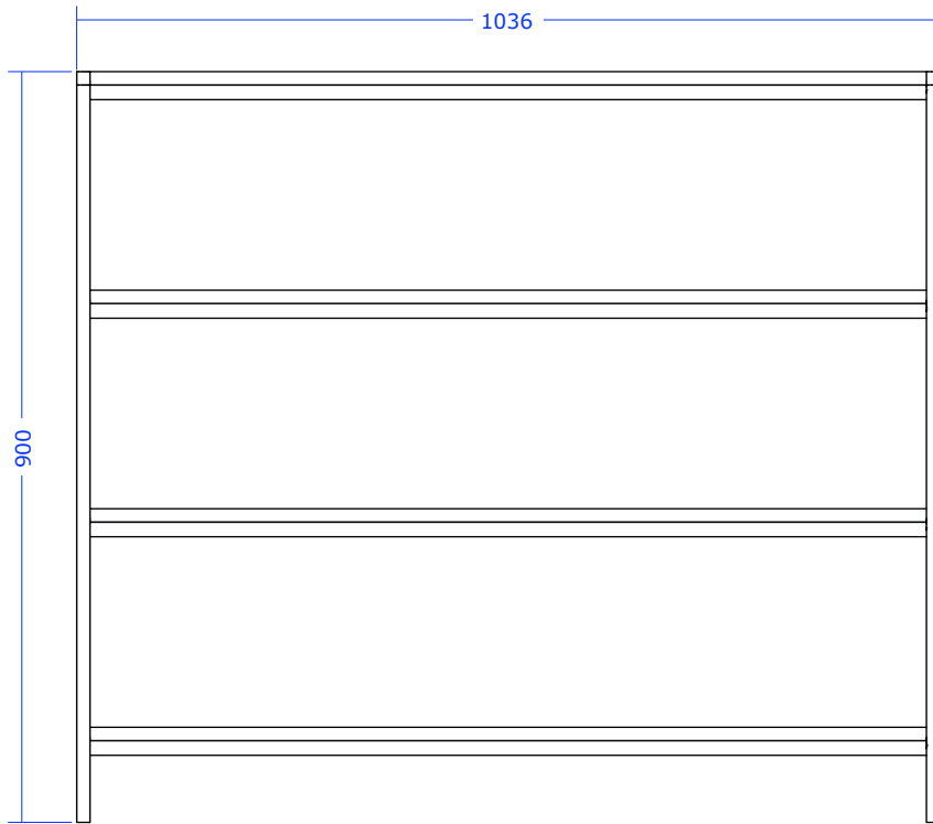
FRONT VIEW
