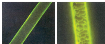
Figure 2: Fluorescence microscope images of the hair after treatment with Gluadin® Soy (1% AS)
