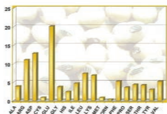
Figure 1: Amino acid profile Gluadin® Soy (relative to amino acid content)
