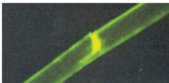
Figure 3: Fluorescence microscope images of the hair fracture site after treatment with Gluadin® Soy (1% AS)
