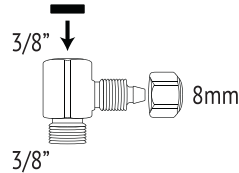
Hot Water T-adapter (3/8" x 3/8" x 8mm)
