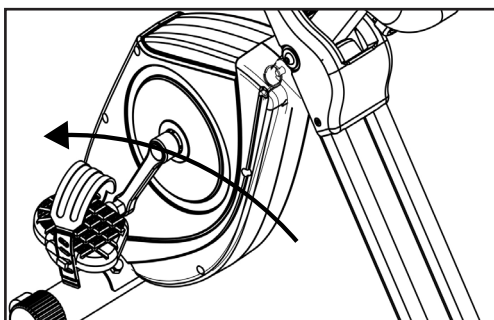
Left pedal assembly
