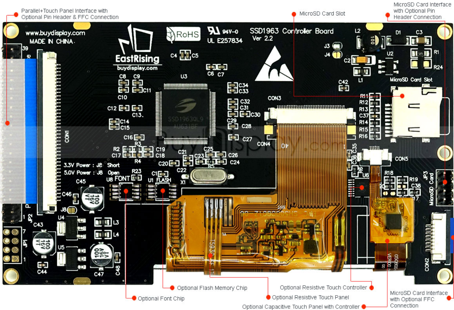
ER-TFTM050-5 Controller Board with Optional Capacitive & Resistive Touch Panel
