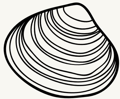
CLAMS
