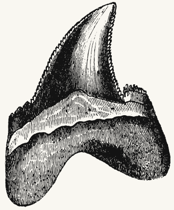
SHARK TOOTH
