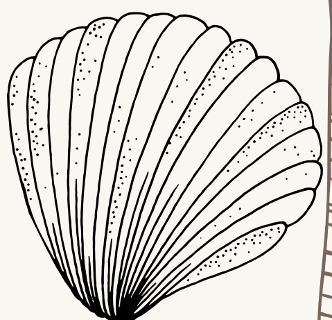
BRACHIOPODS
