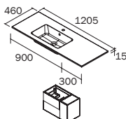
48"/1205 mm Right/Droite (36"+12"/900+300 mm)
