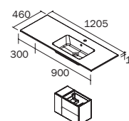
48"/1205 mm Left/Gauche (12"+36"/300+900 mm)
