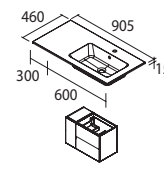
36"/905 mm Left/Gauche (12"+24"/300+600 mm)
