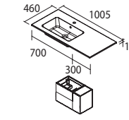
40"/1005 mm Right/Droite (28"+12"/700+300 mm)
