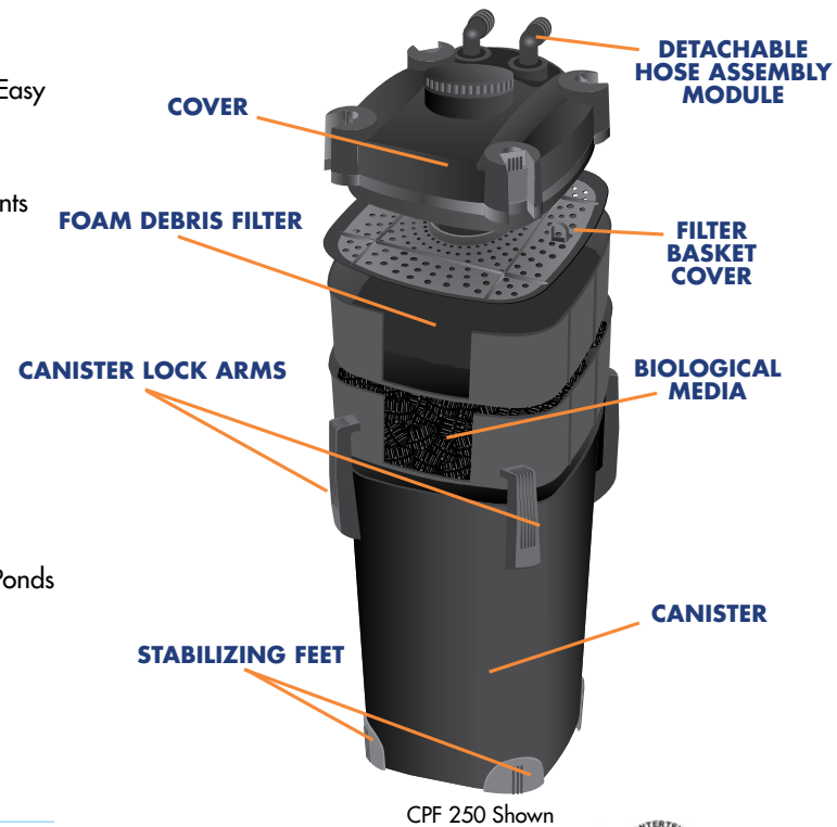
CPF 250 Shown
