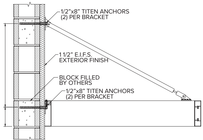
E.F.I.S. OVER CMU BLOCK WALL
