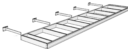
EXPLODED VIEW
