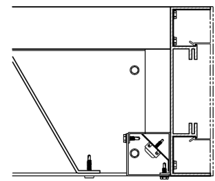
Z-BLADE WITH FRONT STRIP LIGHTING
