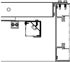
RAIN PAN STRIP LIGHTING
