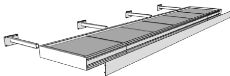
EXPLODED VIEW
