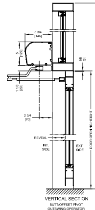
GT710 Operator
