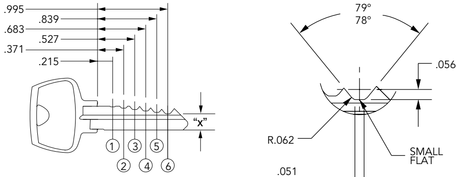
6 PIN POSITIONS Shown, depth and spacing are the same for 5 & 7 pin
