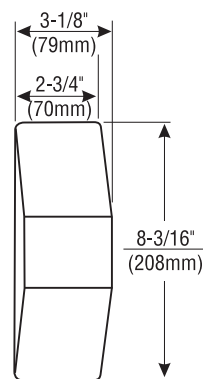
Cover Detail
