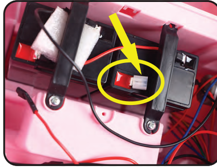
8. Pull out the white insulating caps.
