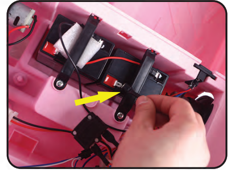
9. Connect the two power terminals.
