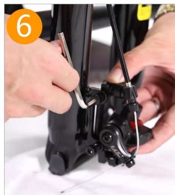
Tighten the first screw
