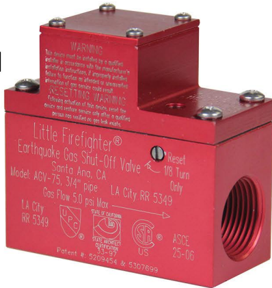
AGV-75 Horizontal
