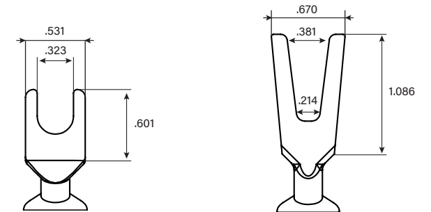
U-Spade Dimensions (in.)
