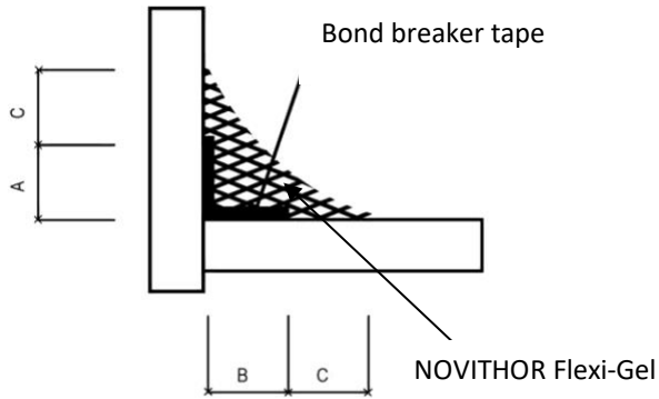
GOOD JOINT DESIGN
