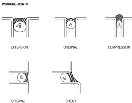
Figure 54 – Working Joints Applications
