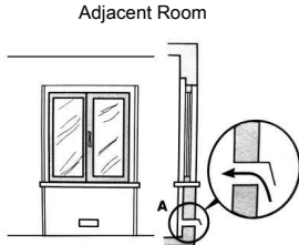
Examples of ventilation holes for comburent air.
