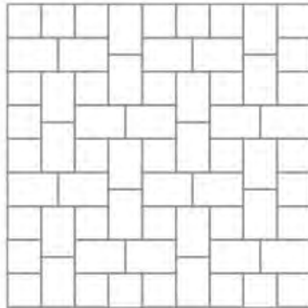
I-PATTERN (25% 6" X 6" + 75% 6" X 9")
