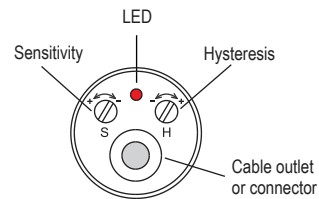
Top view of level sensor
