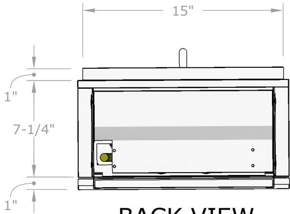
BACK VIEW SCALE 1:7
