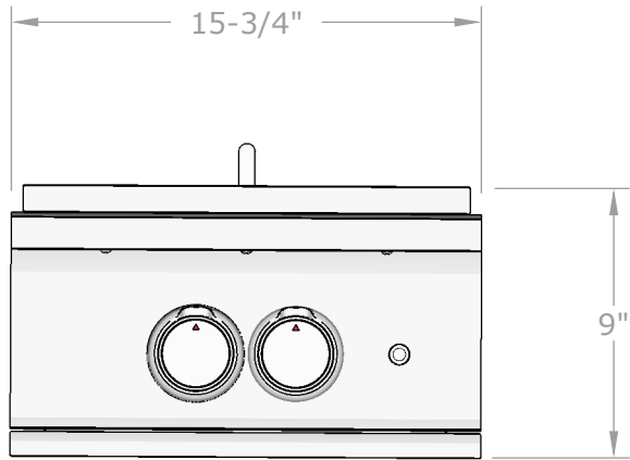
FRONT VIEW SCALE 1:7
