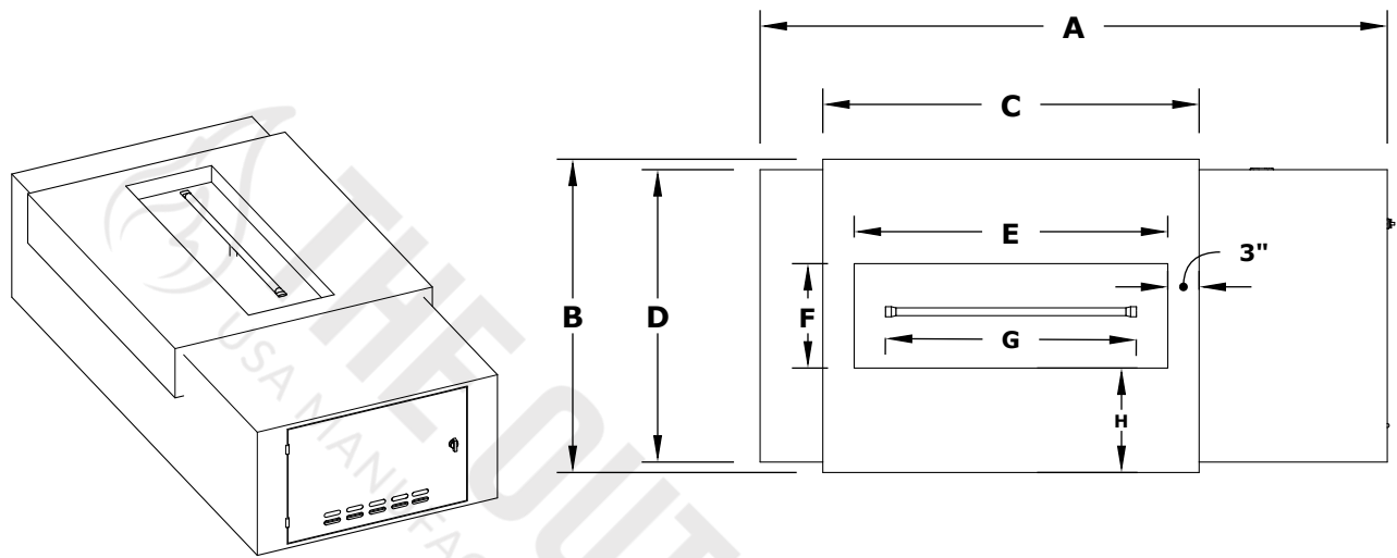
ISOMETRIC VIEW
