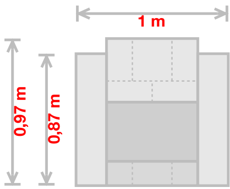
top view closed position
