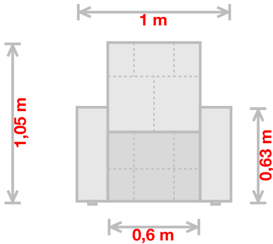
front view closed position
