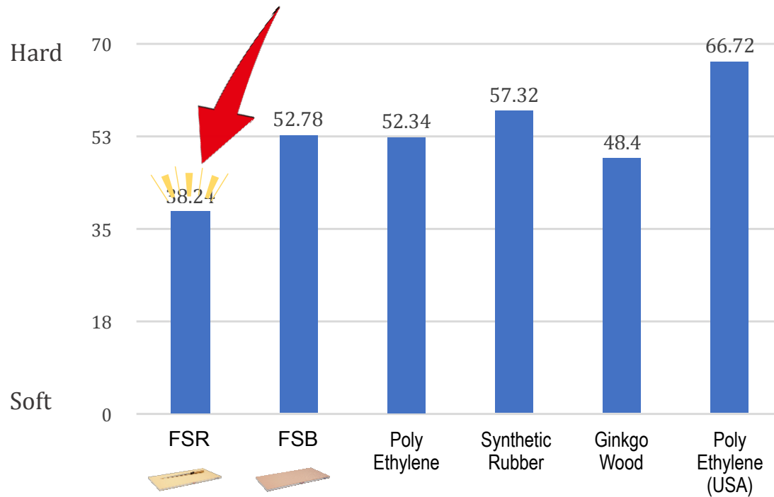
Figure 1. Average hardness of different cutting boards
