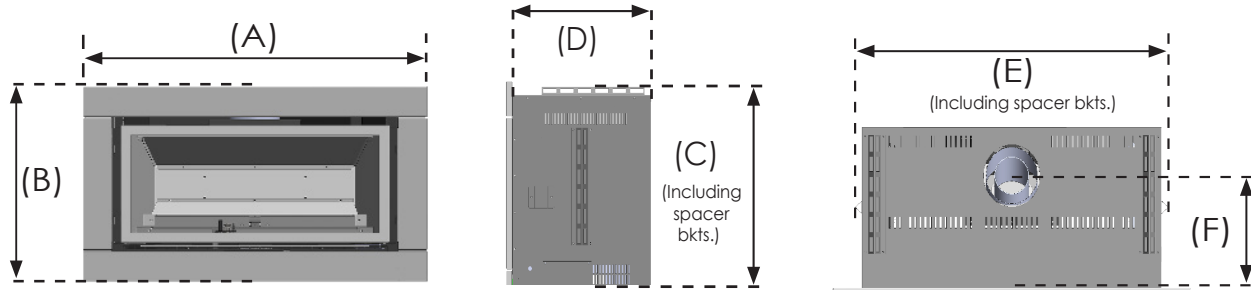
External dimensions for all Luminar Inbuilt Gas Log Fires (All dimensions in millimeters)
