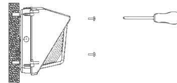
Step 8: Put back the upper cover on the base plate and fixing two screws
