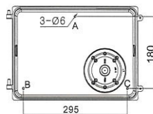
Step 4: Drill the holes on the base plate, according to A, B, C position (Unit: mm)
