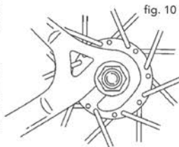
Bolt-on Rear Wheel in Dropouts
