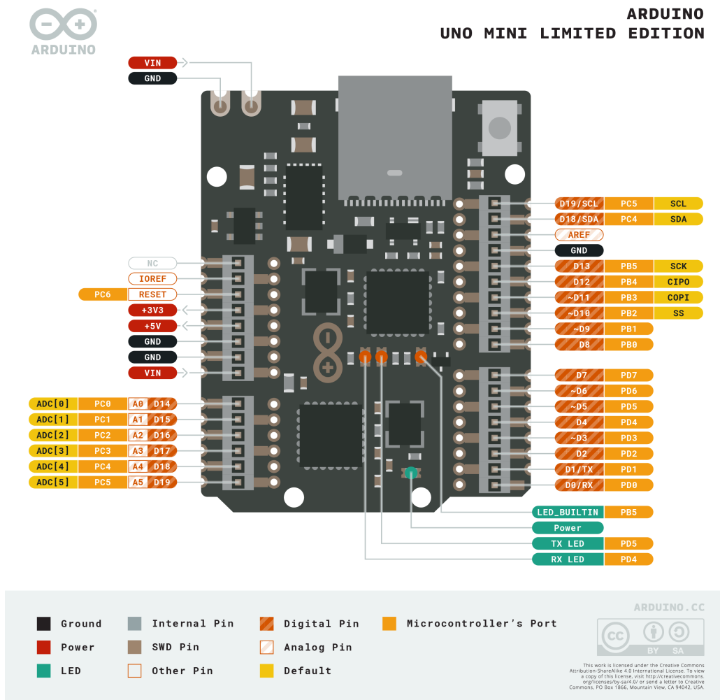
Pinout
